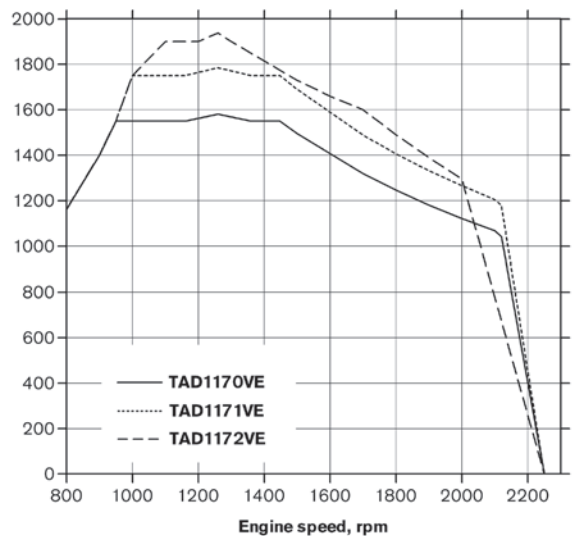
Torque, Nm
